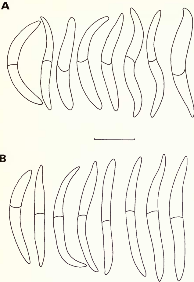
Fig. 9 Ascospore outlines (A) Leptorhaphis epidermidis (Ach.) Th. Fr. (UPS-ACH 001669b-isolectotype); (B) H-NYL 7503-holotype of Verrucaria oxyspora ; scale = 10 \mu m.
